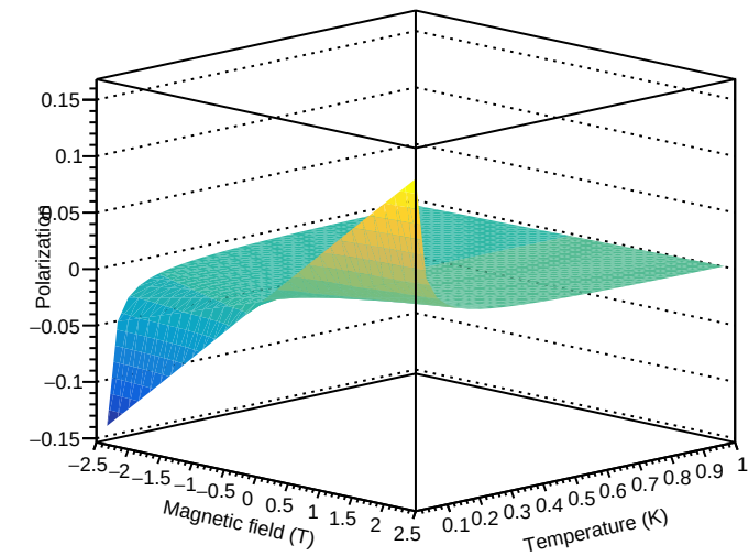
Polarization as a function of magnetic field and temperature
