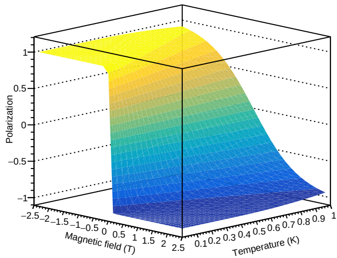
Polarization as a function of magnetic field and temperature
