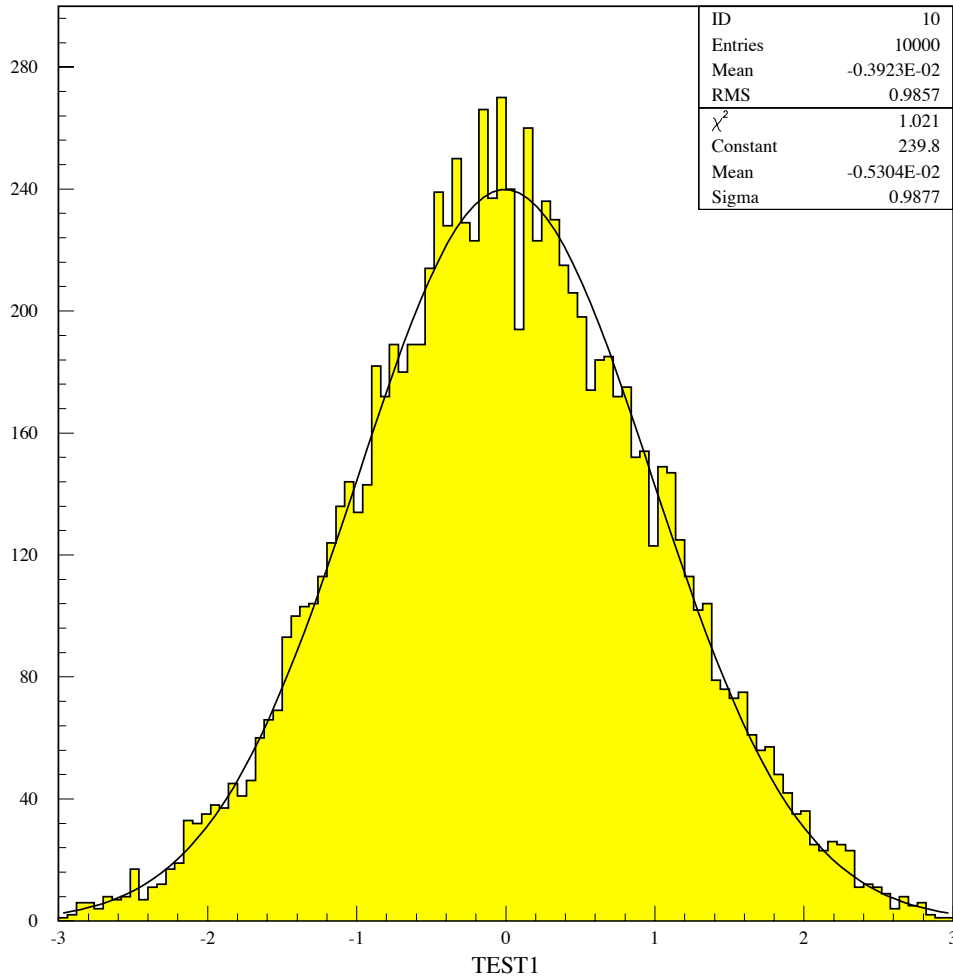
Figure 6.9: Example of a simple fit of a one-dimensional distribution
