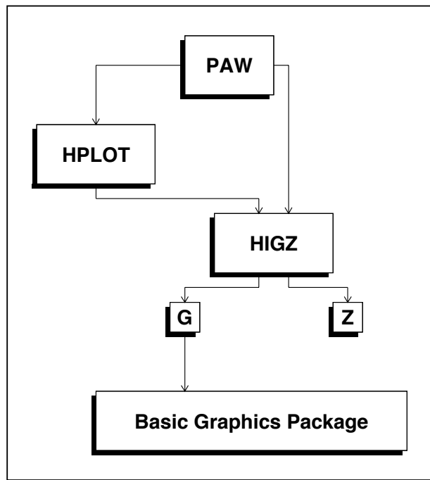
Figure 7.1: HPILOT and HIGZ in PAW
