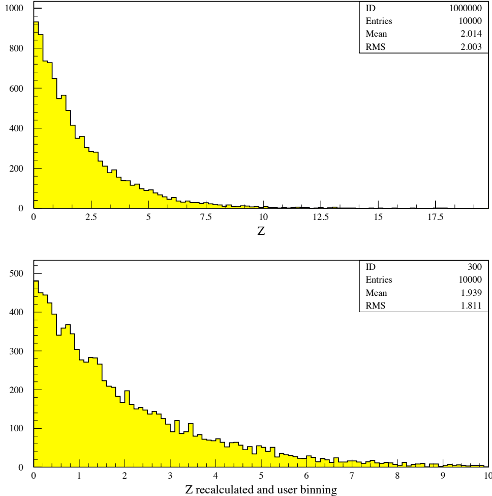
Figure 6.7: Read and plot Ntuple elements
