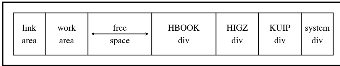
Figure 6.1: The layout of the /PAWC/ dynamic store
