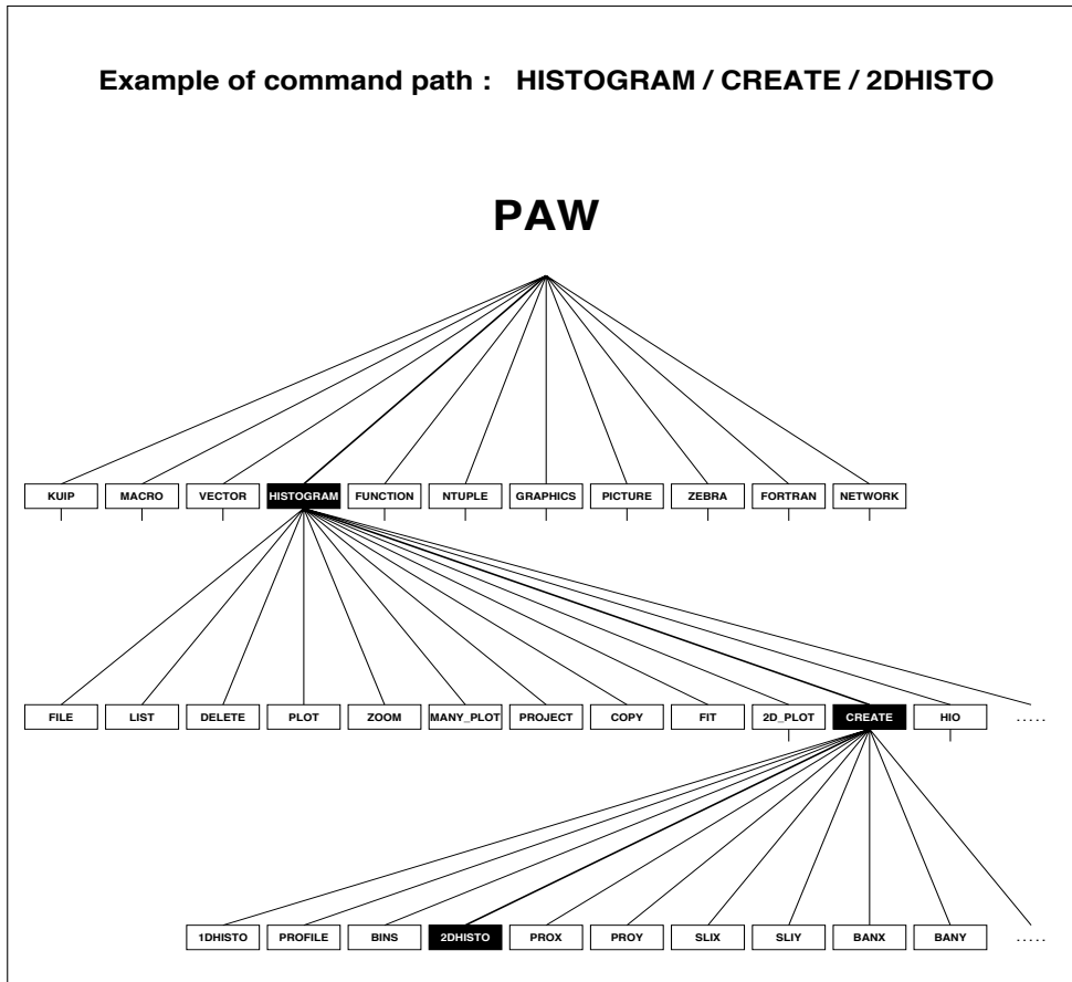
Figure 3.1: Example of the PAW command tree structure
