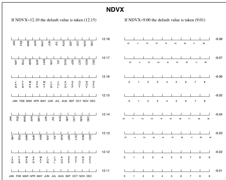
Figure 7.4: Example of labelling for horizontal axes
